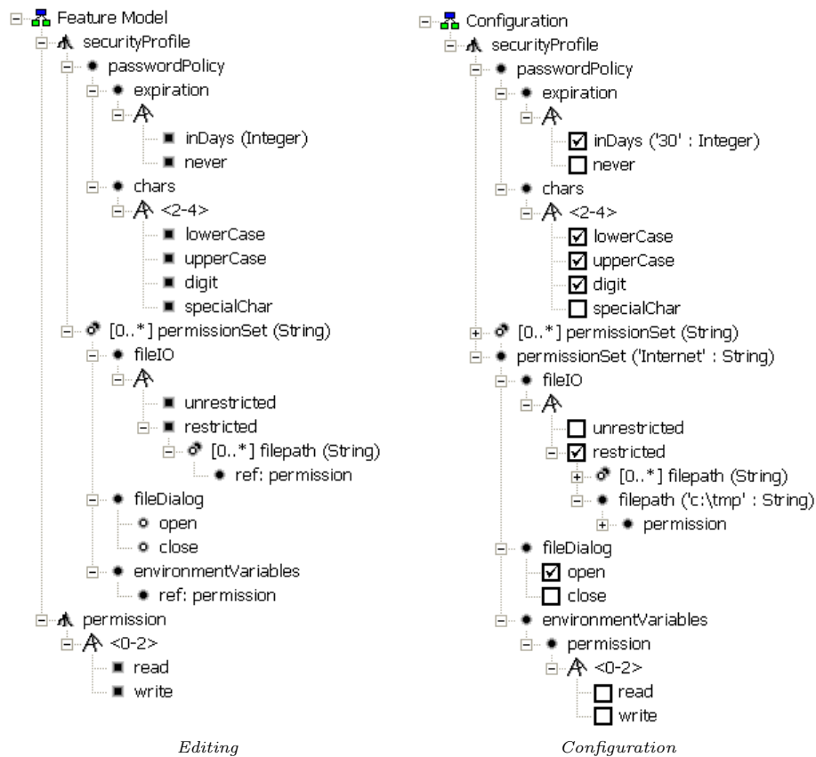
Figure 7. Example of feature model editing and configuration interface
