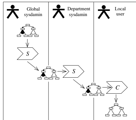
Figure 4. SPEM model for staged configuration of policy standards
