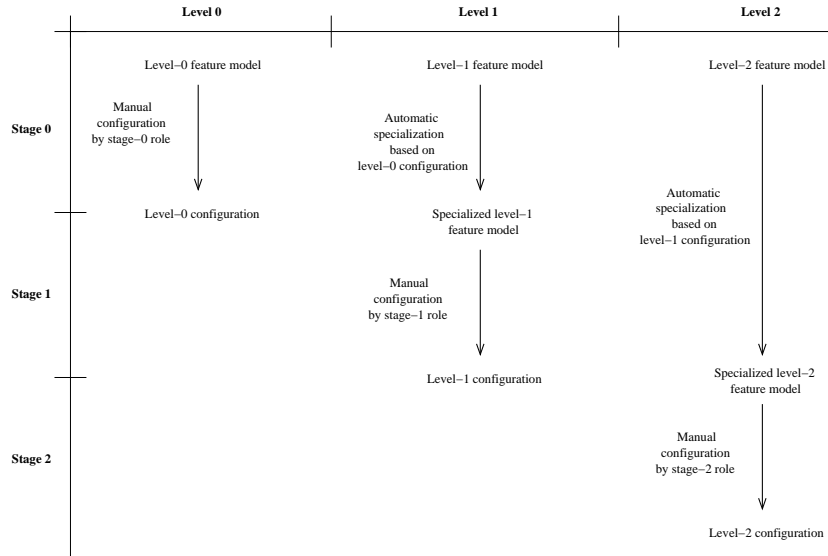
Figure 10. Three-level configuration
