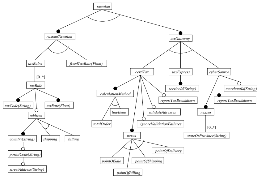
Level-1 feature diagram (system level)
