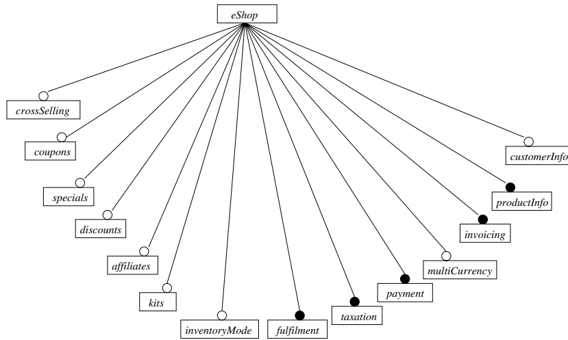
Level-0 feature diagram (product-line level)
