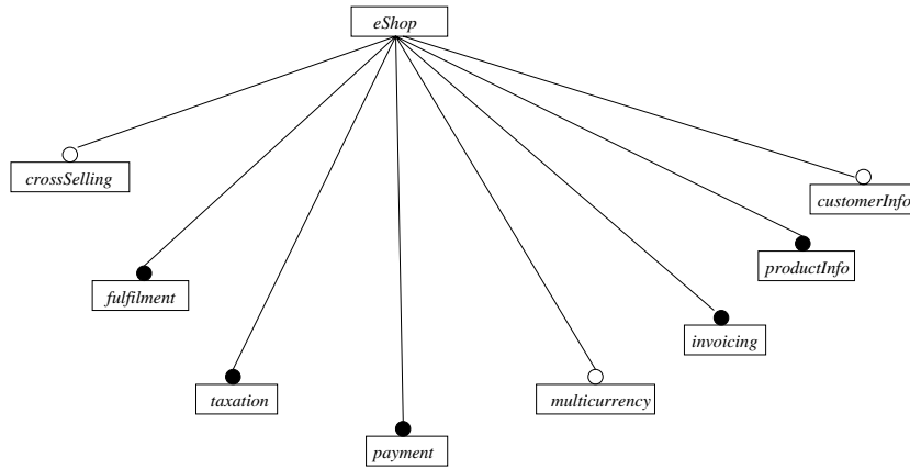
Level-1 feature diagram (system level)
