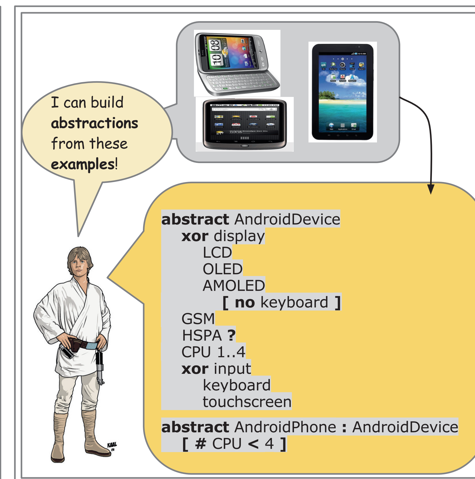
Abstraction inference from examples
