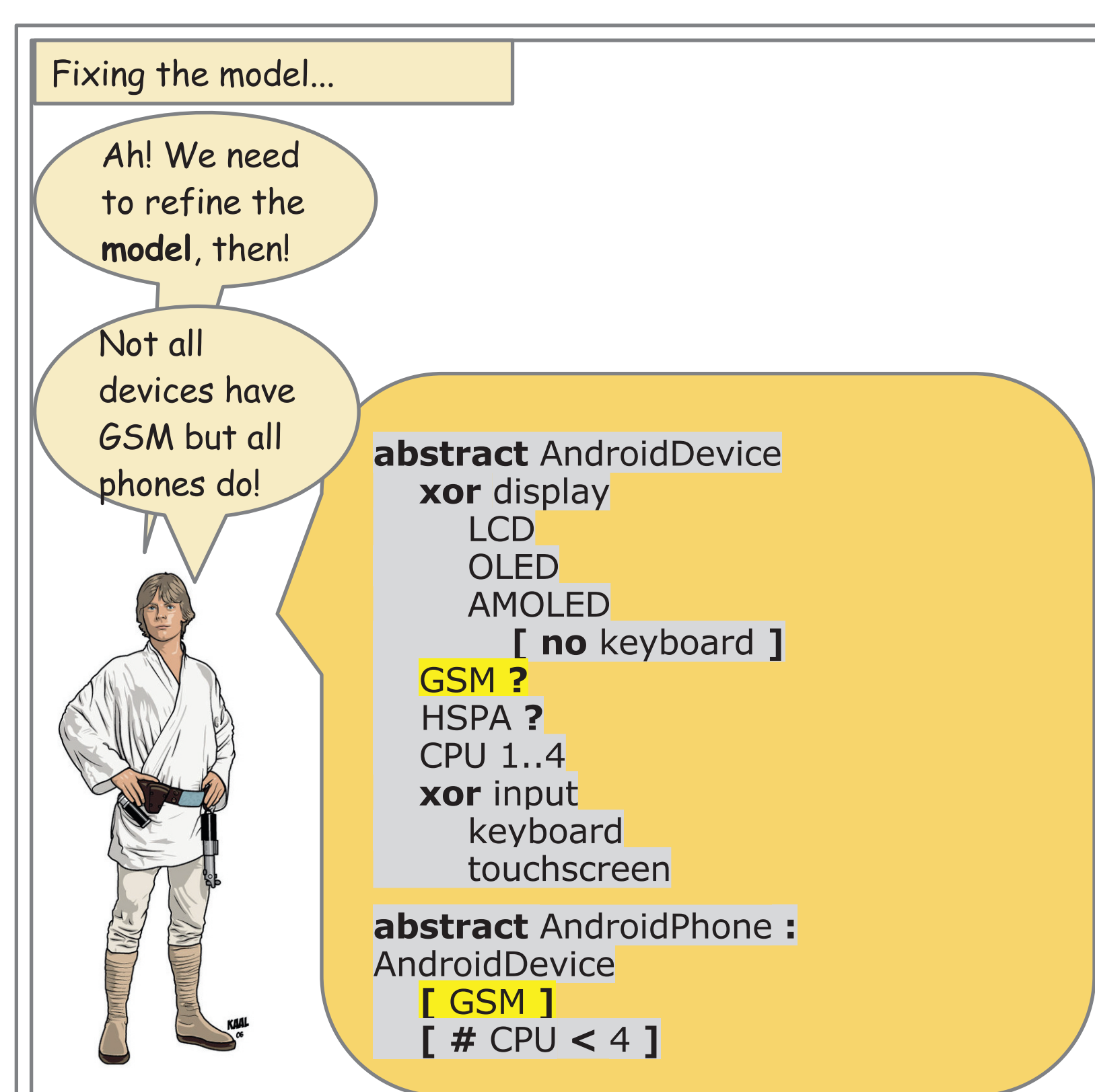
Model refinement based on feedback
