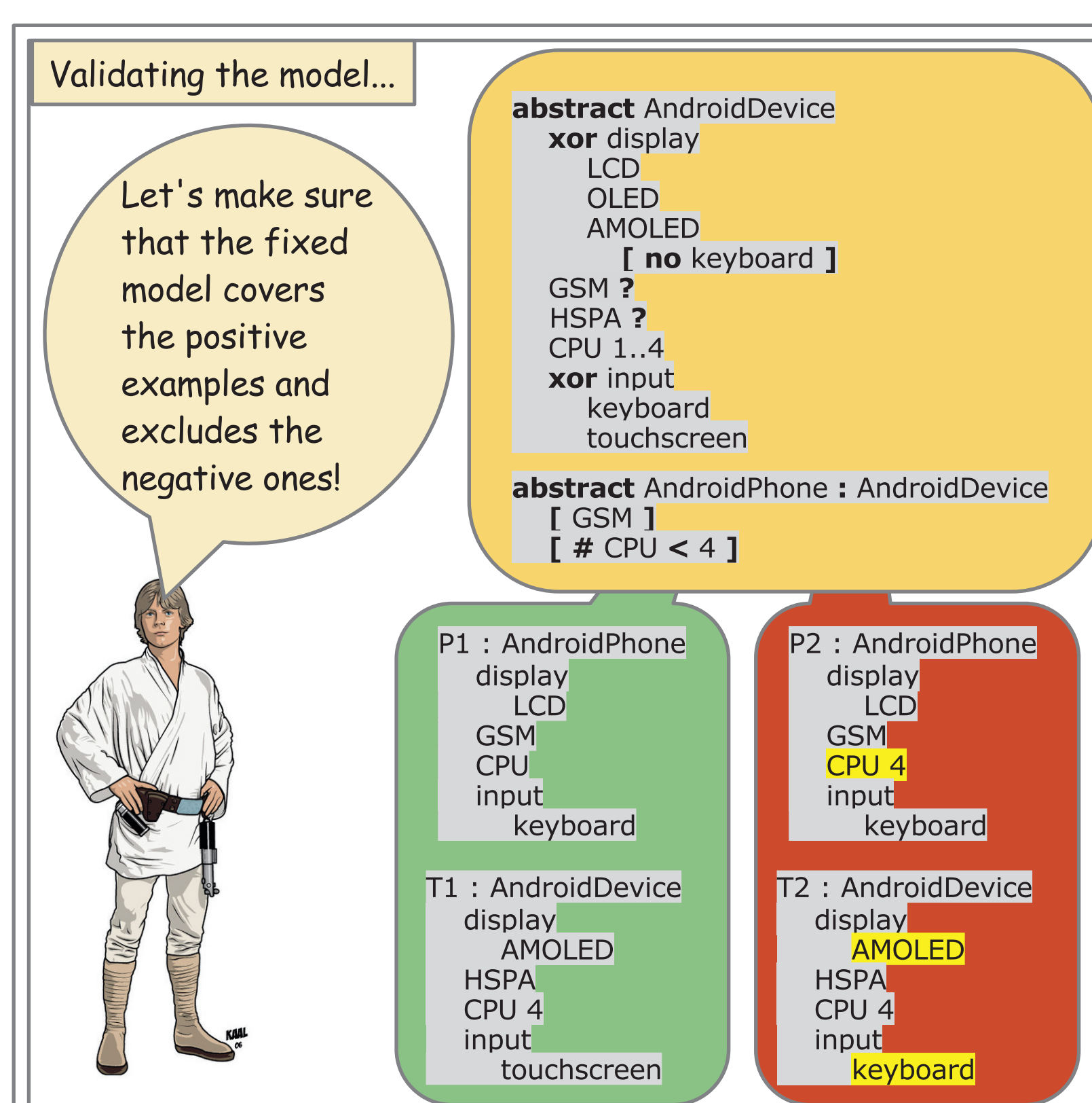
Model validation using examples
